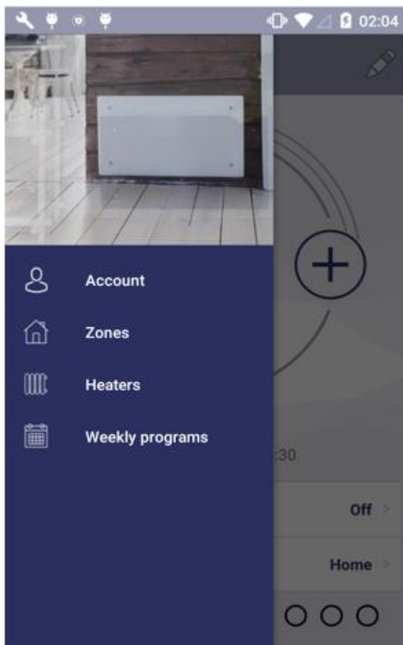
Figure 15. Menu window
