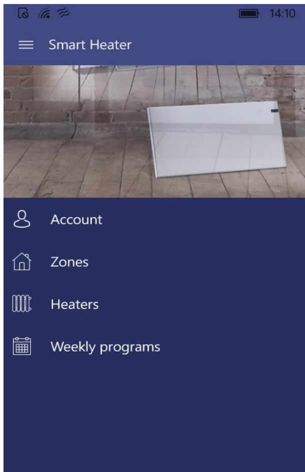
Figure 28. Menu window
