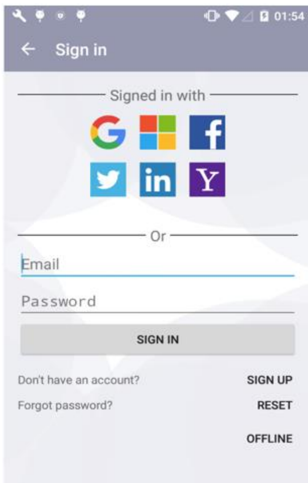
Figure 13. Login screen
