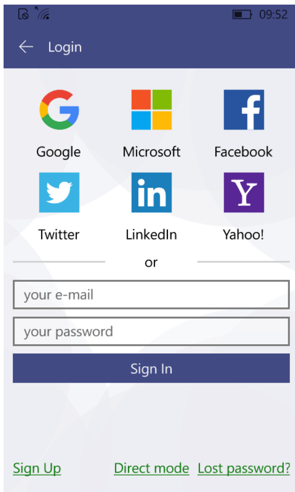
Figure 26. Login screen
